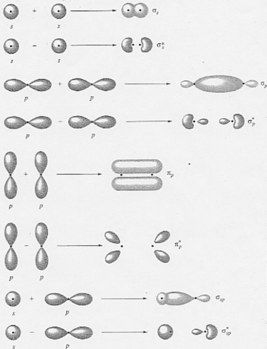
Figure 8.31 Molecular orbitals that result from the allowed combinations (addition and subtraction) of s and p atomic orbitals. Each set of two orbitals forms one bonding and one antibonding molecular orbital.
